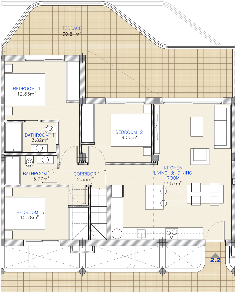
VIVIENDA SEGUNDA PLANTA + SOLARIUM SECOND FLOOR HOUSING + SOLARIUM
